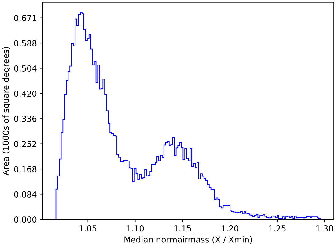
ddf_loaded_fl1_v3.4_10yrs All sky z band: Median normairmass
