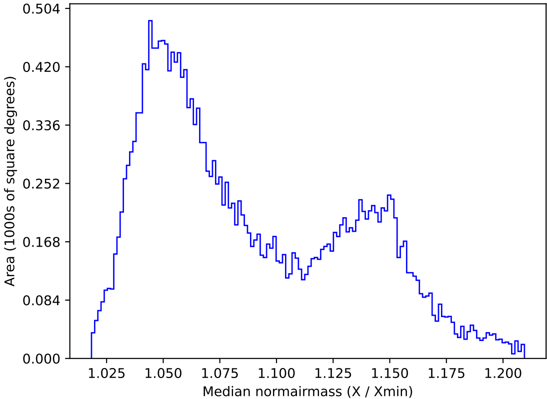
ddf_loaded_fl1_v3.4_10yrs All sky y band: Median normairmass
