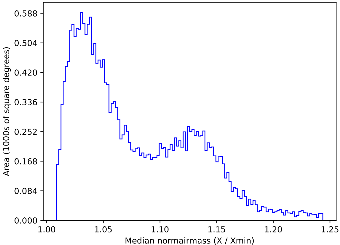
ddf_loaded_fl1_v3.4_10yrs All sky u band: Median normairmass
