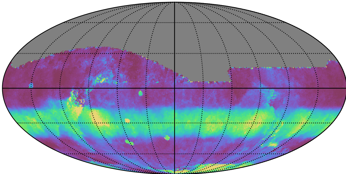
ddf_loaded_fl1_v3.4_10yrs All sky r band: Median normairmass
