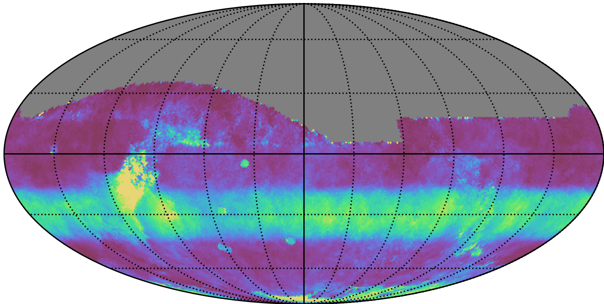
ddf_loaded_fl1_v3.4_10yrs All sky i band: Median normairmass
