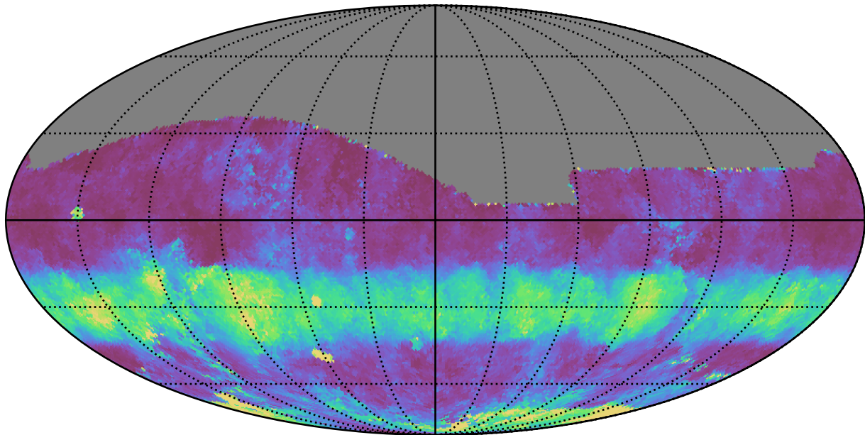
ddf_loaded_fl1_v3.4_10yrs All sky g band: Median normairmass
