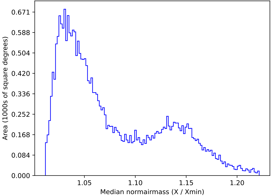
ddf_loaded_fl1_v3.4_10yrs All sky g band: Median normairmass
