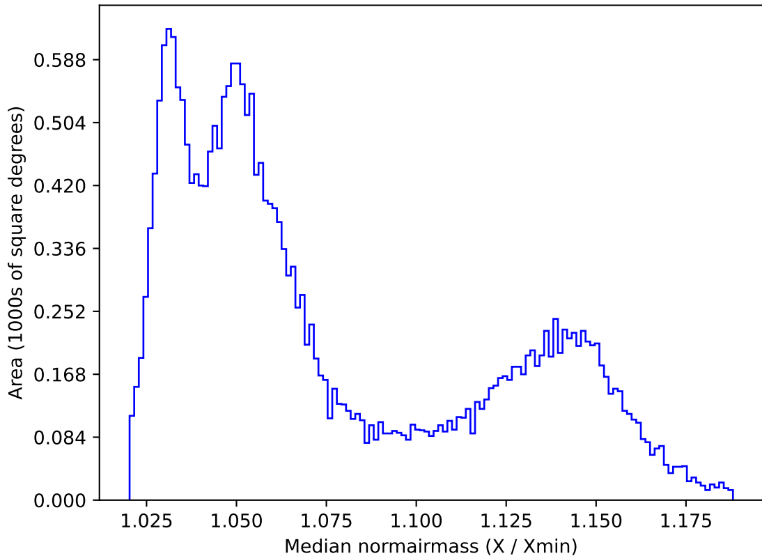
ddf_loaded_fl1_v3.4_10yrs All sky all bands: Median normairmass
