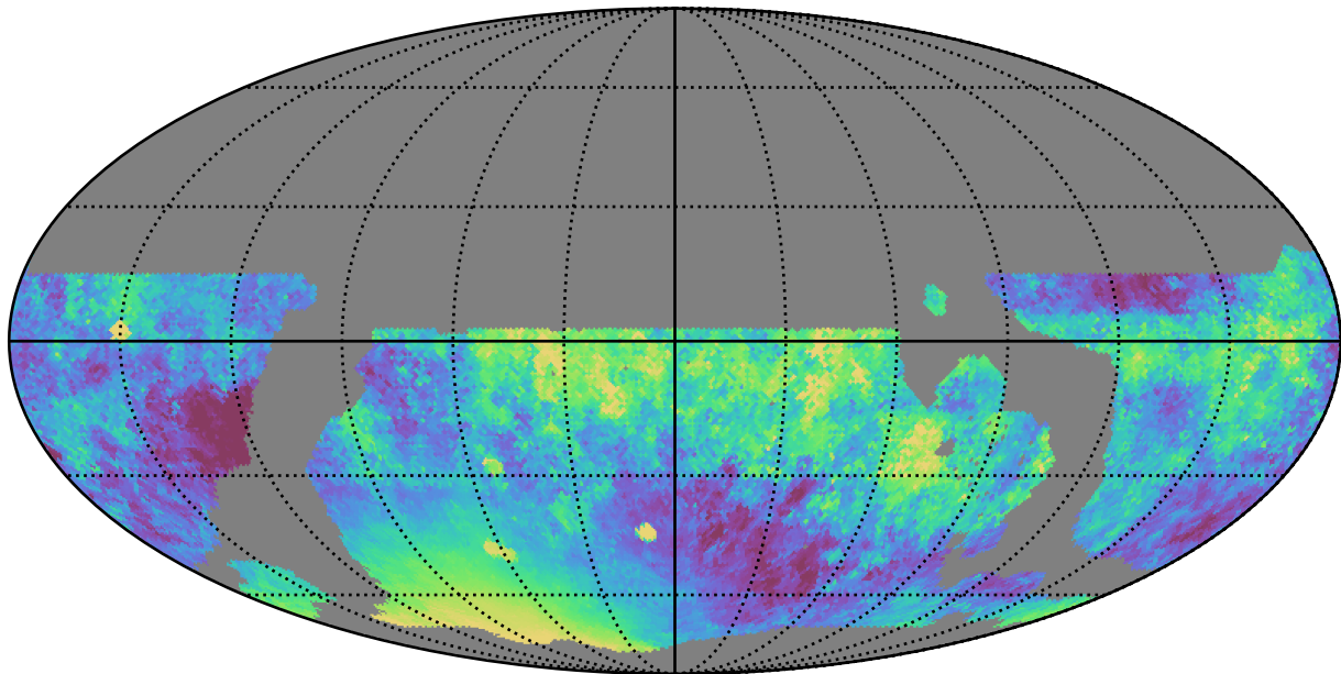
ddf_loaded_fl1_v3.4_10yrs WFD z band: Median moonDistance
