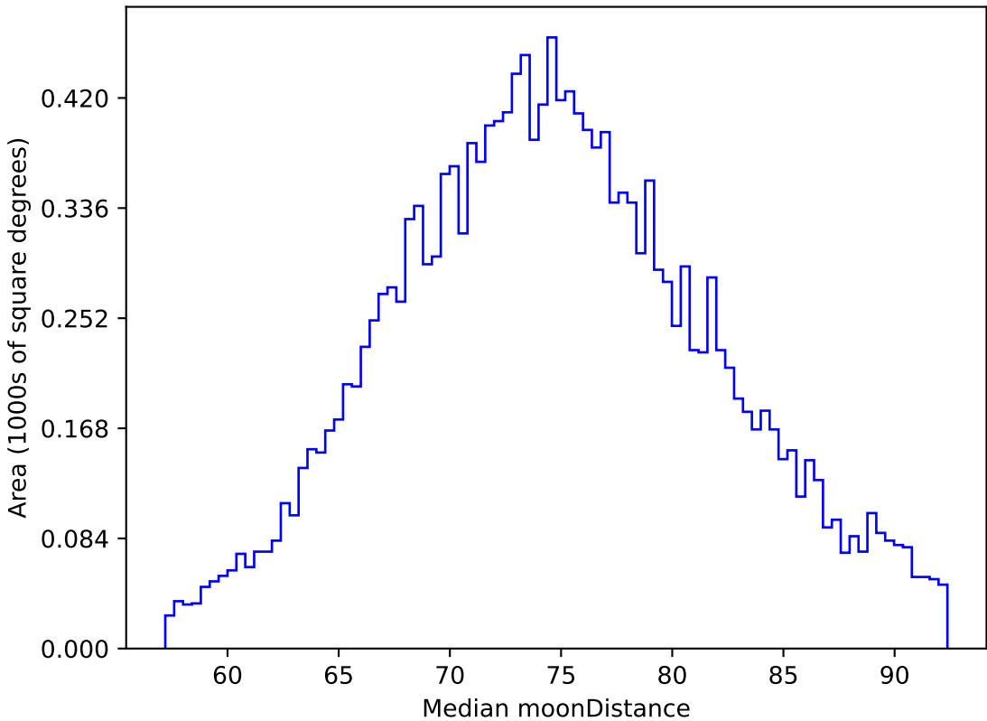
ddf_loaded_fl1_v3.4_10yrs WFD z band: Median moonDistance
