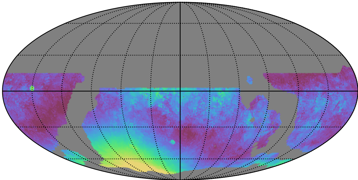
ddf_loaded_fl1_v3.4_10yrs WFD y band: Median moonDistance
