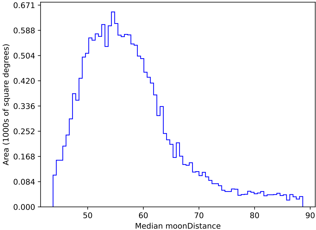
ddf_loaded_fl1_v3.4_10yrs WFD y band: Median moonDistance
