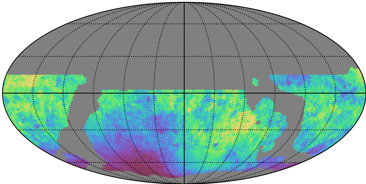
ddf_loaded_fl1_v3.4_10yrs WFD r band: Median moonDistance
