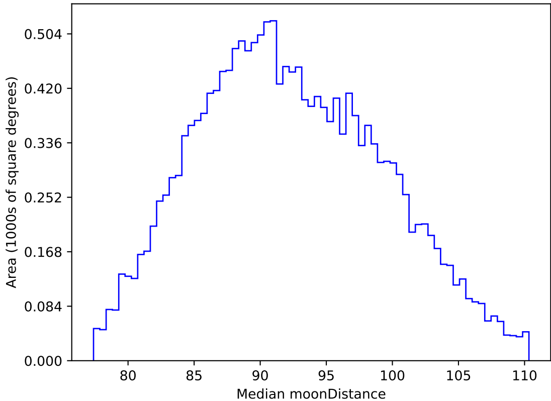
ddf_loaded_fl1_v3.4_10yrs WFD i band: Median moonDistance
