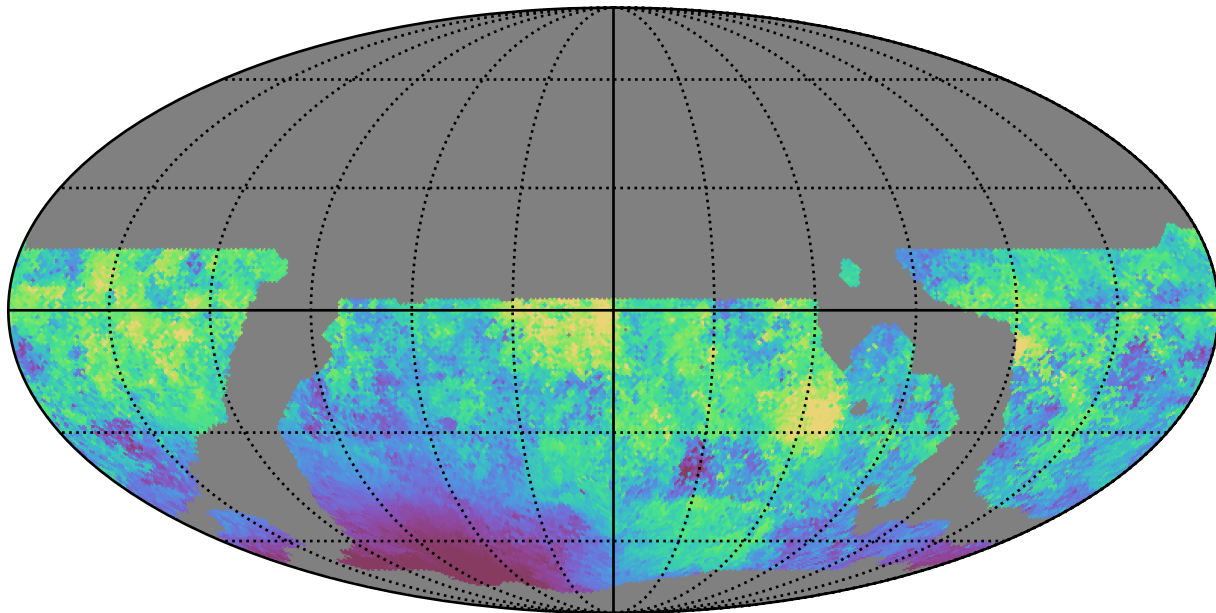
ddf_loaded_fl1_v3.4_10yrs WFD g band: Median moonDistance
