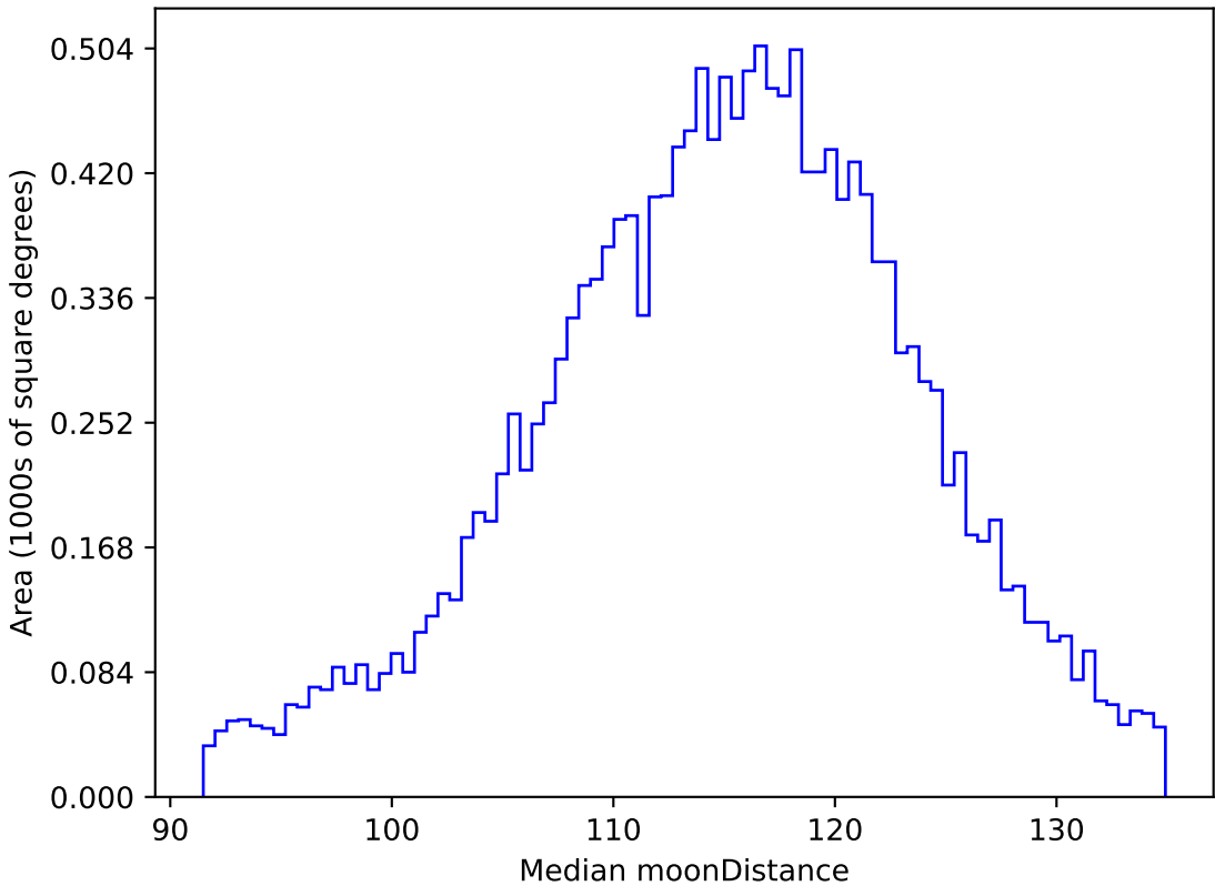
ddf_loaded_fl1_v3.4_10yrs WFD g band: Median moonDistance
