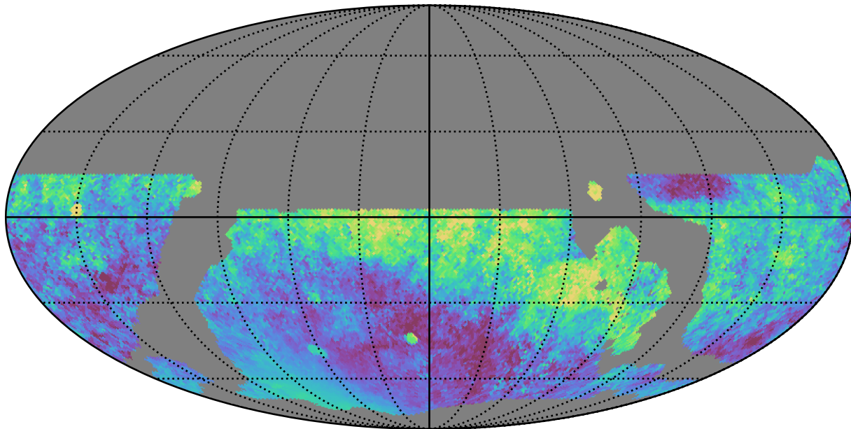
ddf_loaded_fl1_v3.4_10yrs WFD all bands: Median moonDistance
