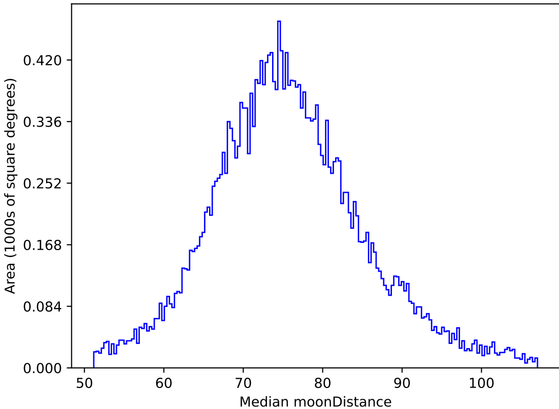
ddf_loaded_fl1_v3.4_10yrs All sky z band: Median moonDistance
