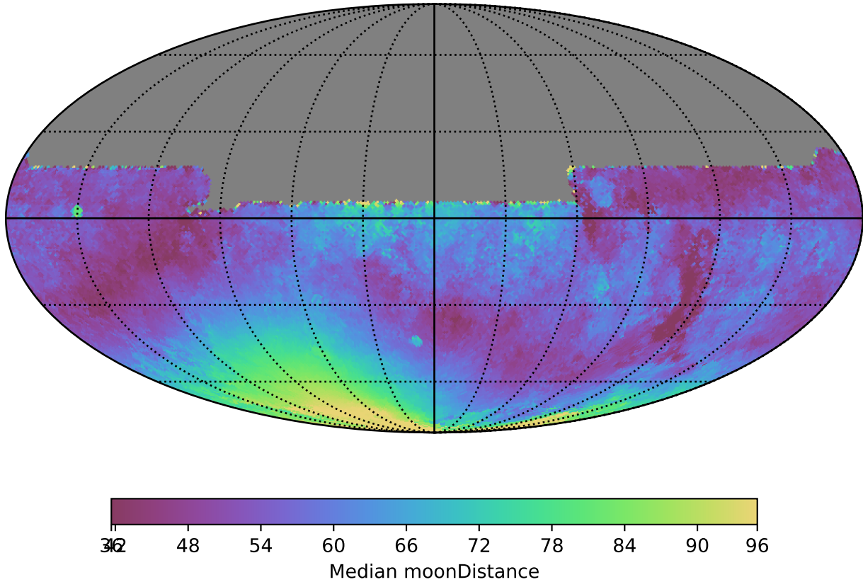
ddf_loaded_fl1_v3.4_10yrs All sky y band: Median moonDistance
