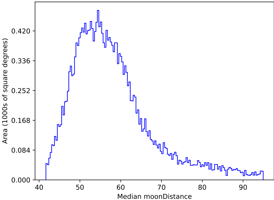
ddf_loaded_fl1_v3.4_10yrs All sky y band: Median moonDistance
