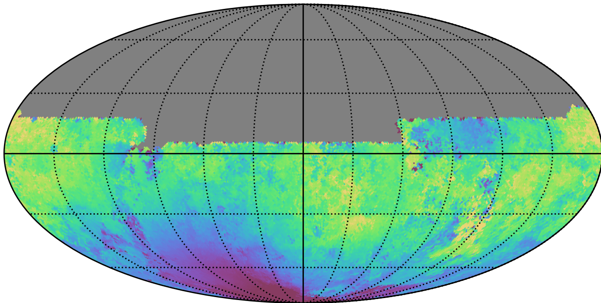
ddf_loaded_fl1_v3.4_10yrs All sky u band: Median moonDistance
