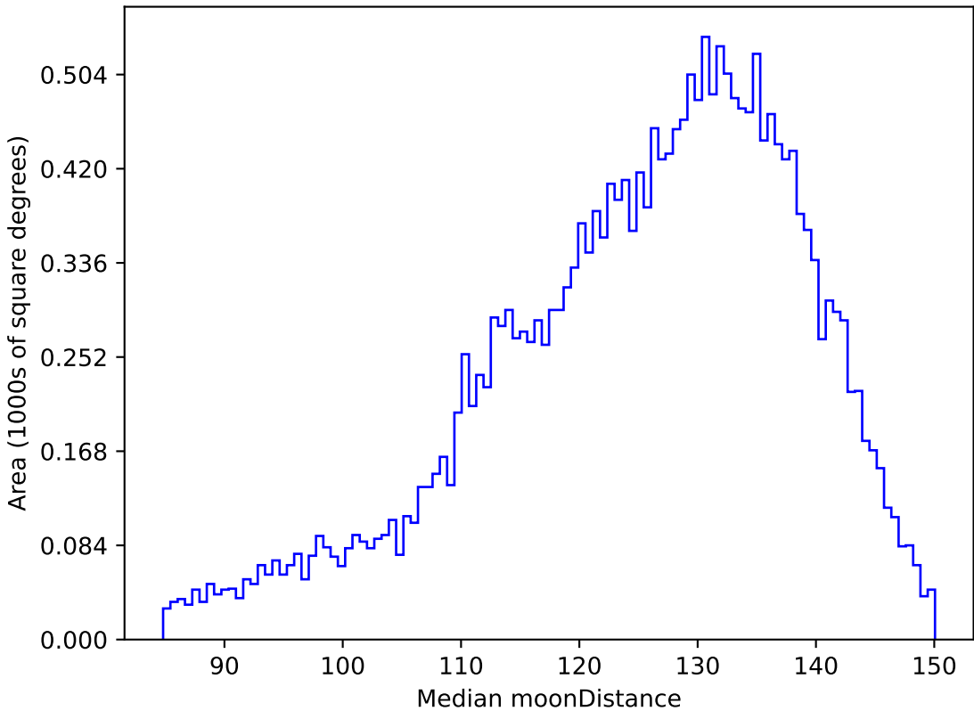
ddf_loaded_fl1_v3.4_10yrs All sky u band: Median moonDistance
