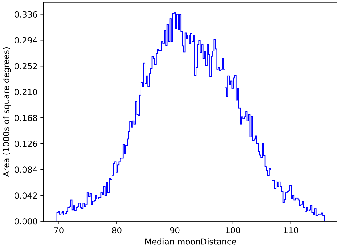
ddf_loaded_fl1_v3.4_10yrs All sky i band: Median moonDistance
