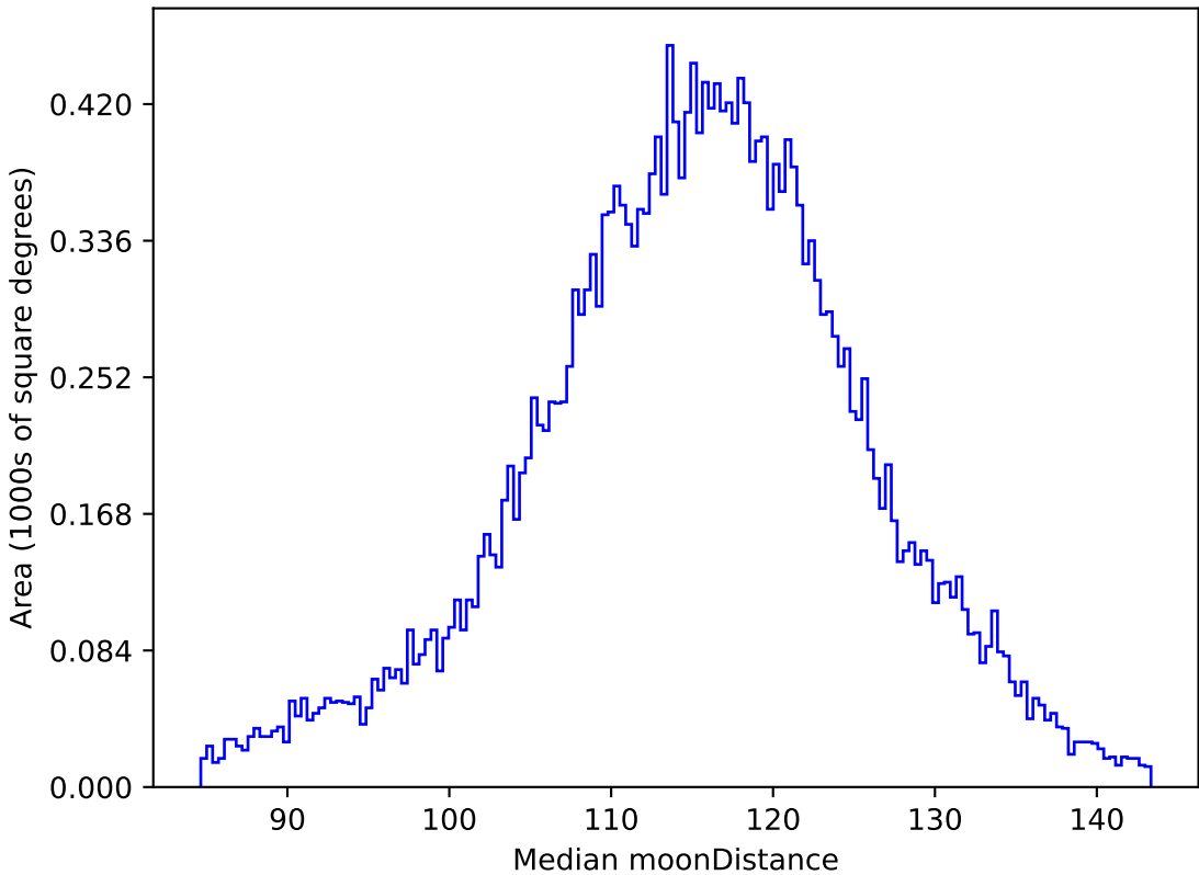
ddf_loaded_fl1_v3.4_10yrs All sky g band: Median moonDistance
