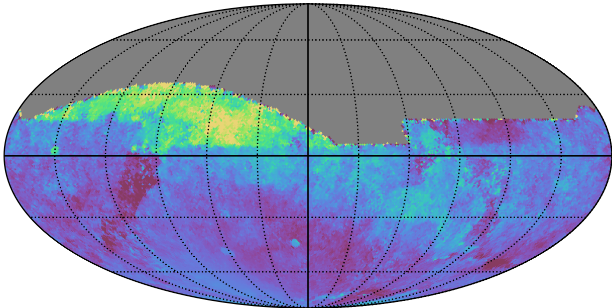
ddf_loaded_fl1_v3.4_10yrs All sky all bands: Median moonDistance
