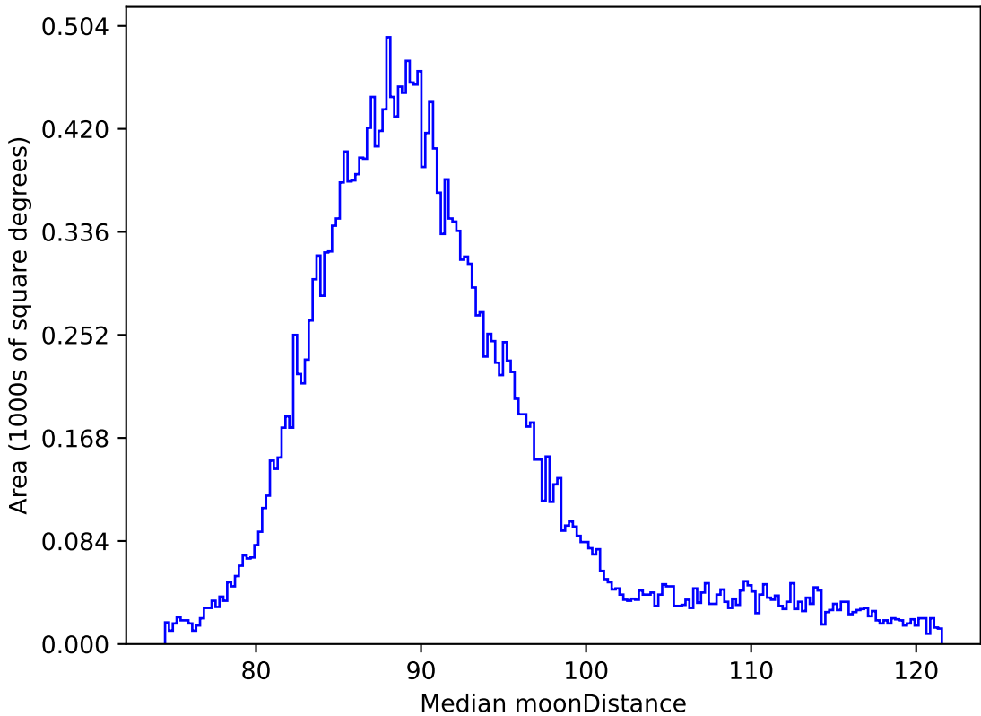
ddf_loaded_fl1_v3.4_10yrs All sky all bands: Median moonDistance
