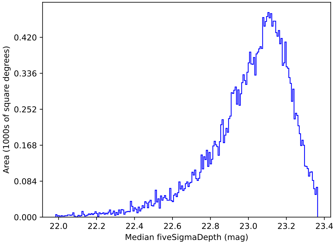
ddf_loaded_fl1_v3.4_10yrs Yr 1 z band: Median fiveSigmaDepth
