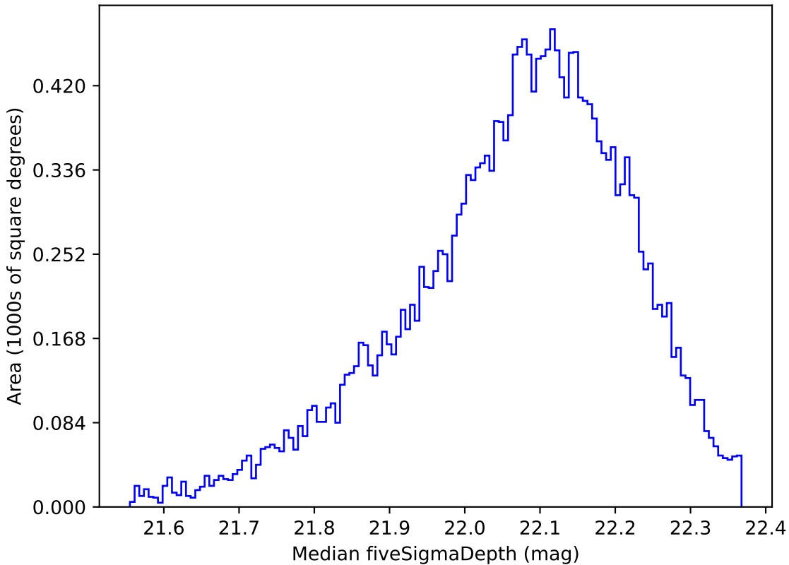
ddf_loaded_fl1_v3.4_10yrs Yr 1 y band: Median fiveSigmaDepth
