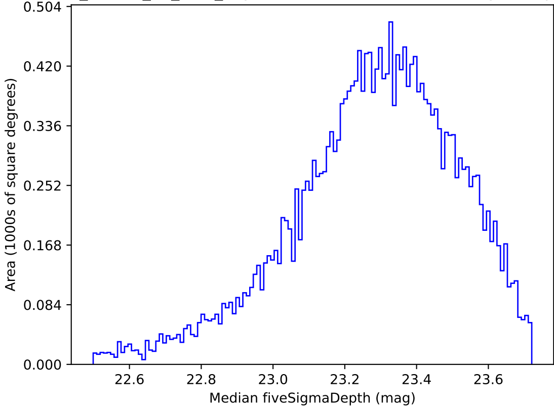
ddf_loaded_fl1_v3.4_10yrs Yr 1 u band: Median fiveSigmaDepth
