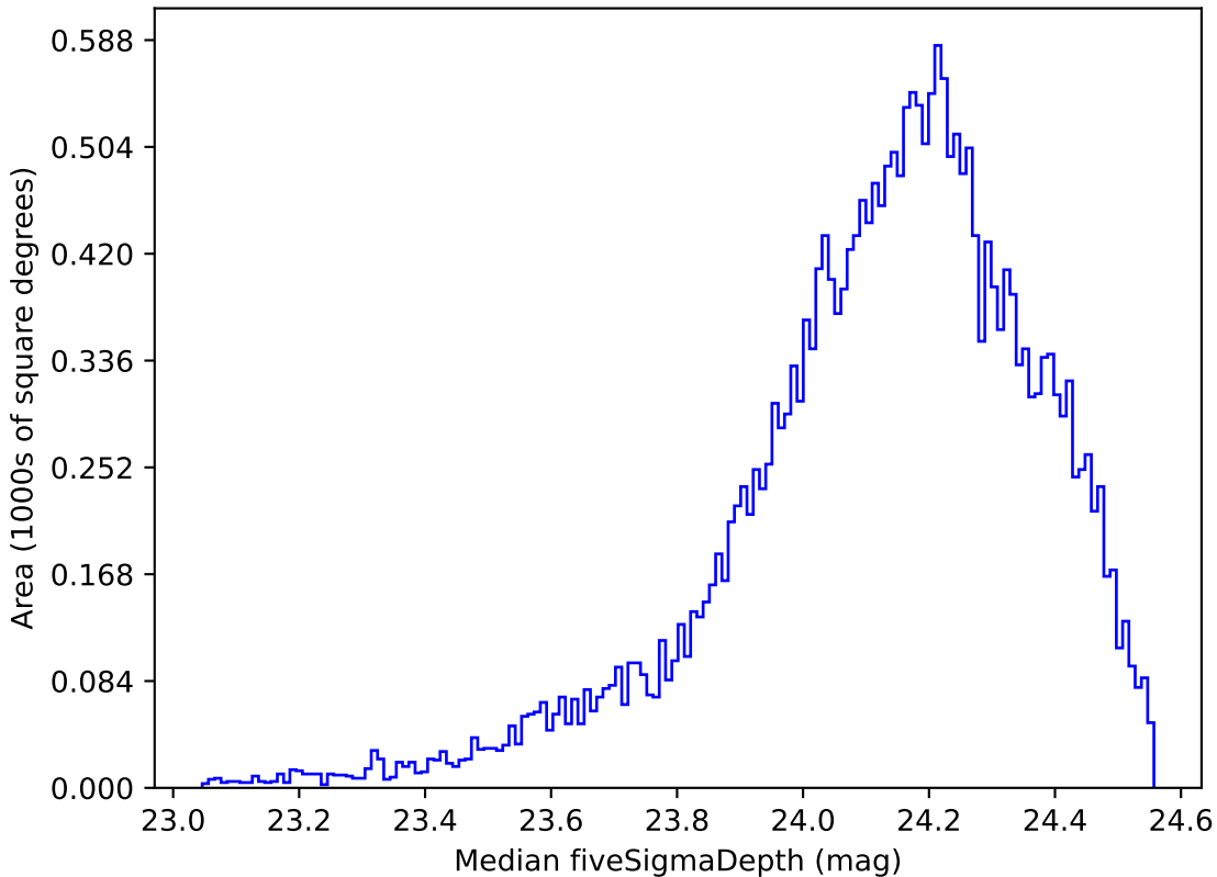
ddf_loaded_fl1_v3.4_10yrs Yr 1 r band: Median fiveSigmaDepth
