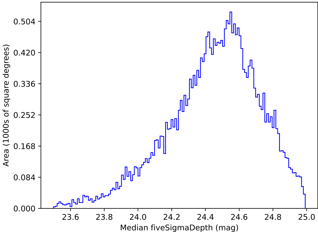
ddf_loaded_fl1_v3.4_10yrs Yr 1 g band: Median fiveSigmaDepth
