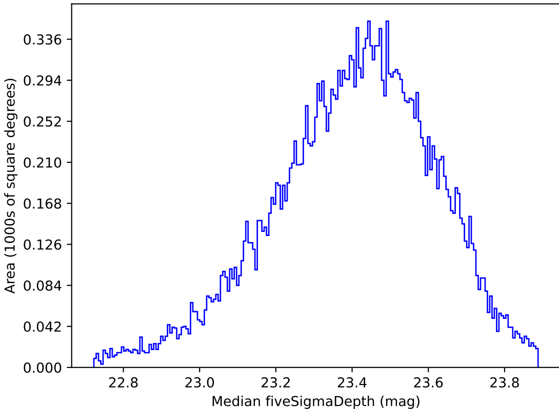
ddf_loaded_fl1_v3.4_10yrs Yr 1 all bands: Median fiveSigmaDepth
