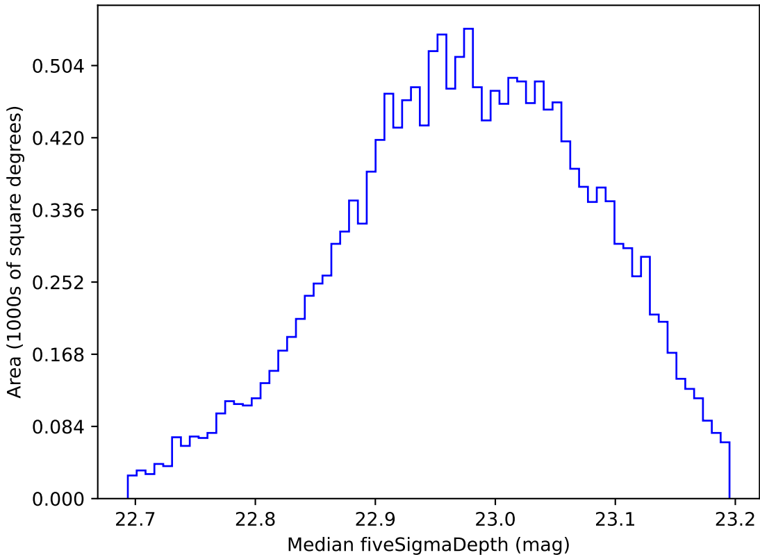
ddf_loaded_fl1_v3.4_10yrs WFD z band: Median fiveSigmaDepth
