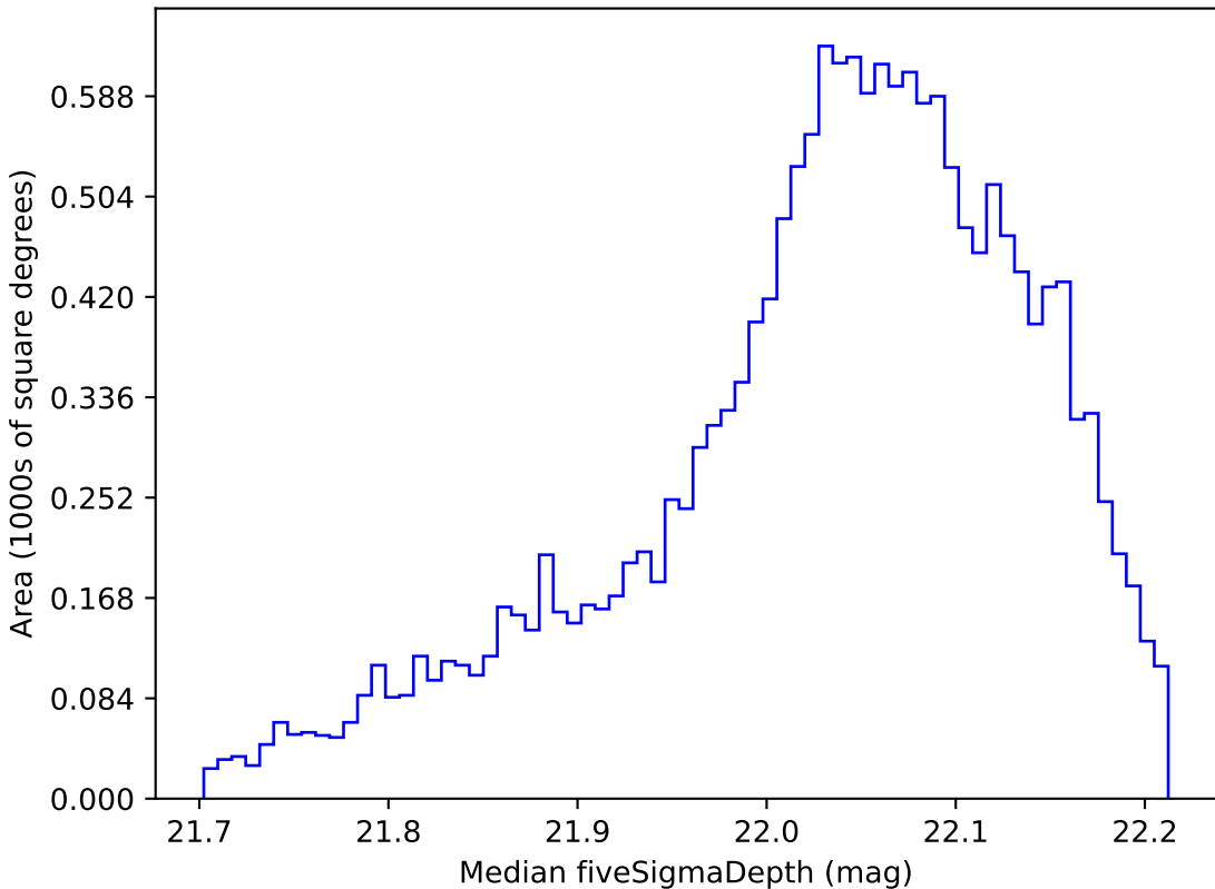
ddf_loaded_fl1_v3.4_10yrs WFD y band: Median fiveSigmaDepth
