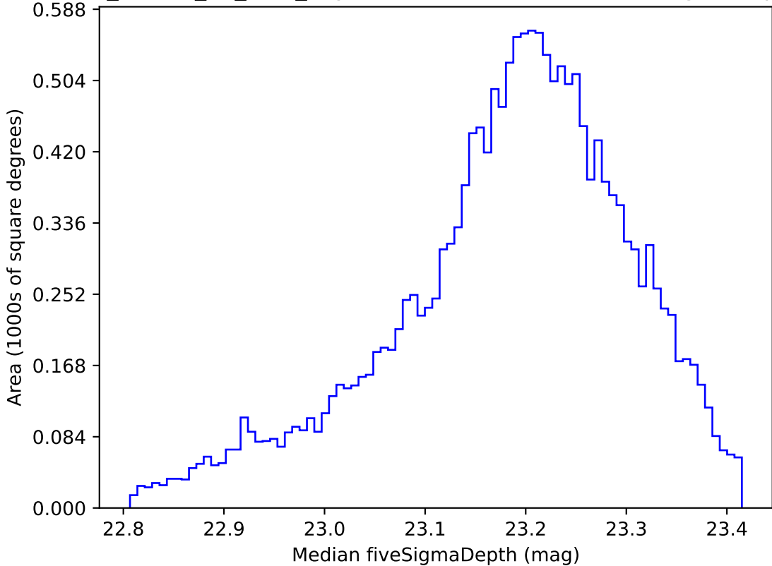
ddf_loaded_fl1_v3.4_10yrs WFD u band: Median fiveSigmaDepth
