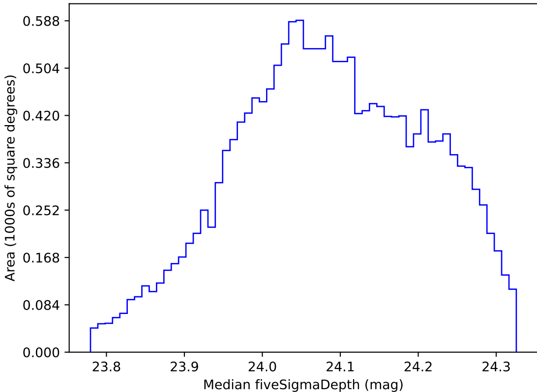
ddf_loaded_fl1_v3.4_10yrs WFD r band: Median fiveSigmaDepth
