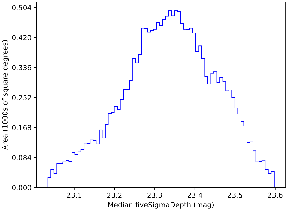
ddf_loaded_fl1_v3.4_10yrs WFD all bands: Median fiveSigmaDepth
