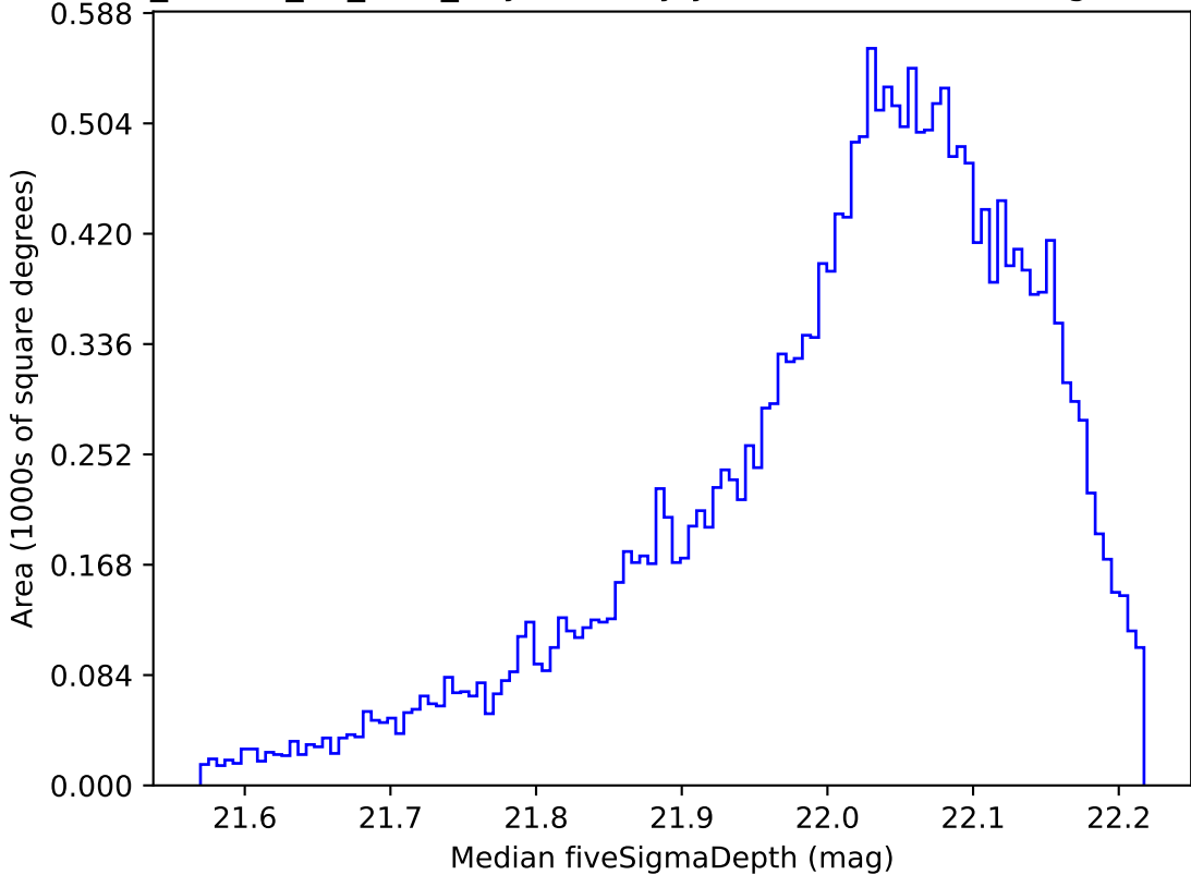
ddf_loaded_fl1_v3.4_10yrs All sky y band: Median fiveSigmaDepth
