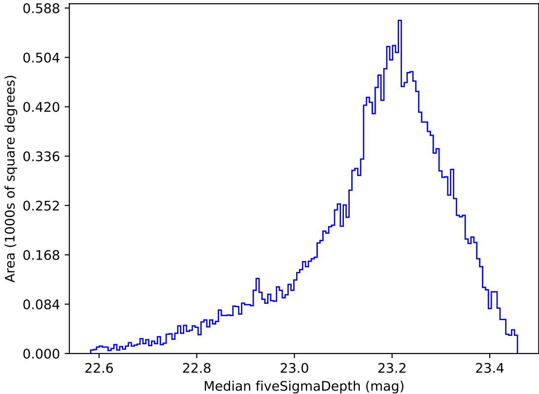
ddf_loaded_fl1_v3.4_10yrs All sky u band: Median fiveSigmaDepth
