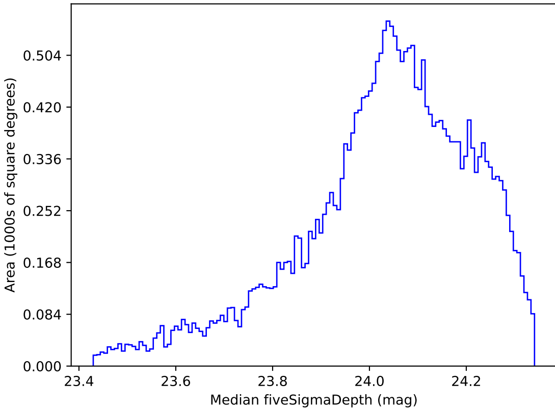
ddf_loaded_fl1_v3.4_10yrs All sky r band: Median fiveSigmaDepth
