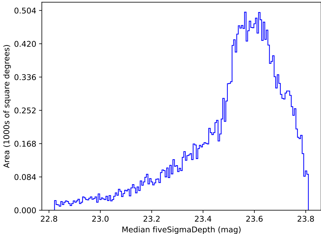
ddf_loaded_fl1_v3.4_10yrs All sky i band: Median fiveSigmaDepth
