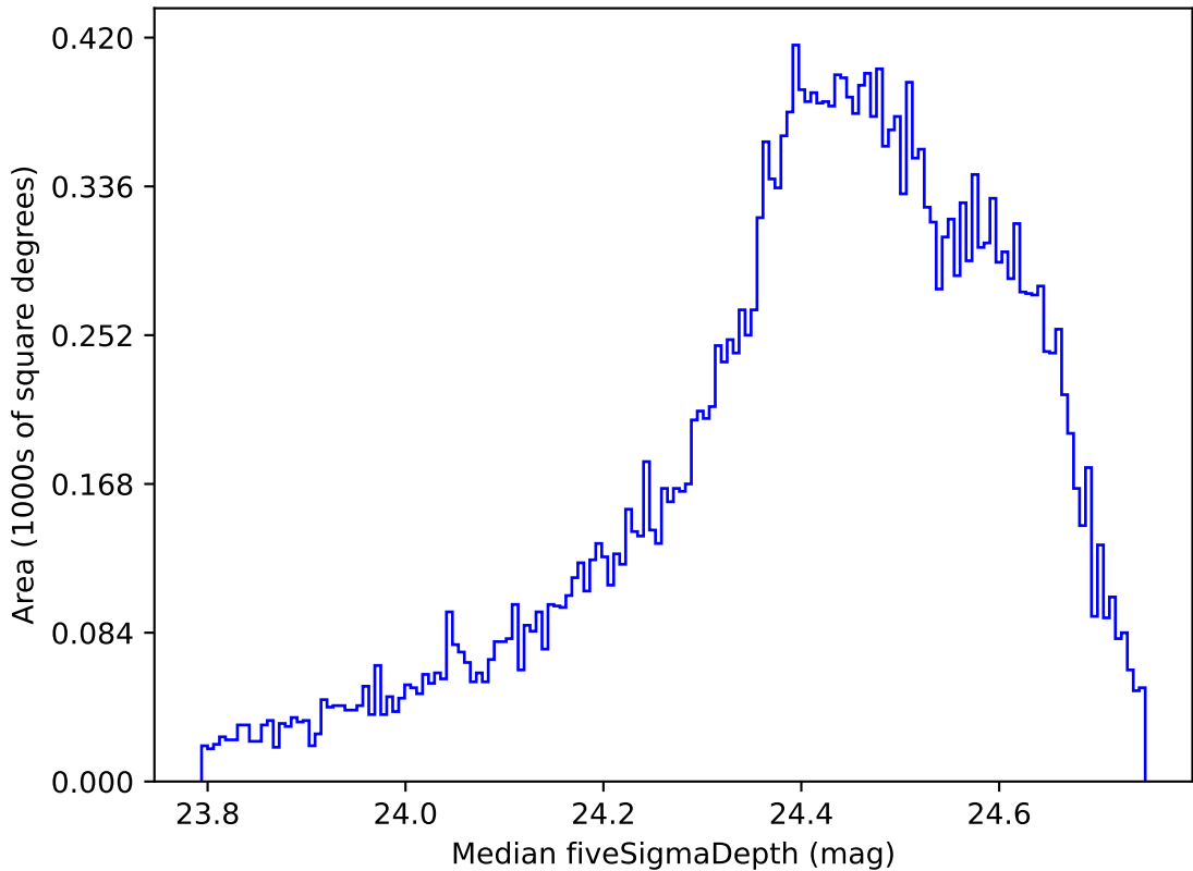
ddf_loaded_fl1_v3.4_10yrs All sky g band: Median fiveSigmaDepth
