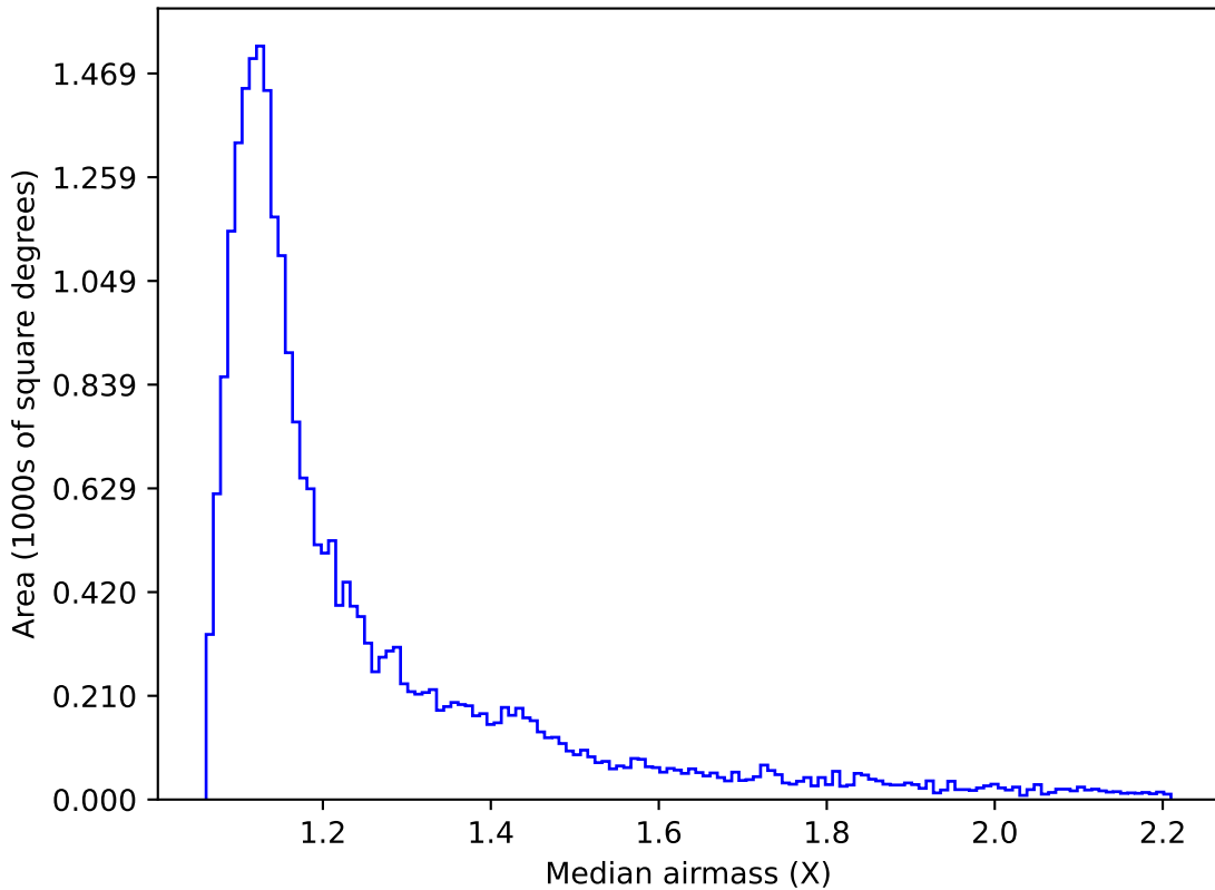
ddf_loaded_fl1_v3.4_10yrs Yr 1 z band: Median airmass
