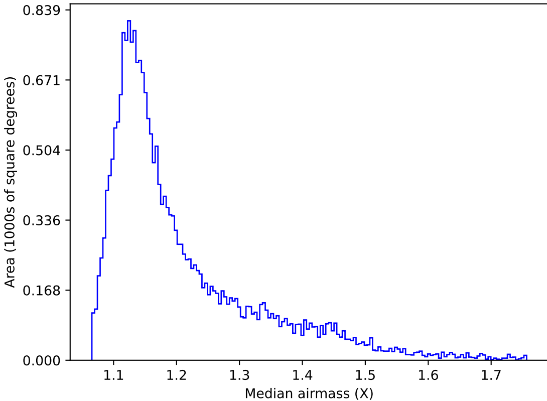
ddf_loaded_fl1_v3.4_10yrs Yr 1 y band: Median airmass
