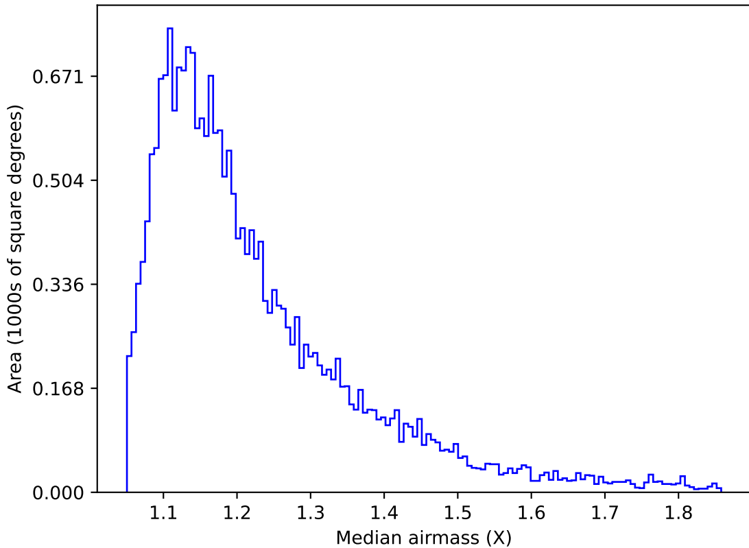
ddf_loaded_fl1_v3.4_10yrs Yr 1 u band: Median airmass
