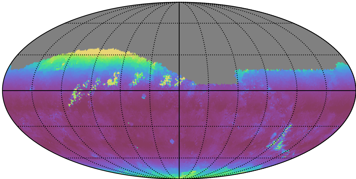
ddf_loaded_fl1_v3.4_10yrs Yr 1 r band: Median airmass
