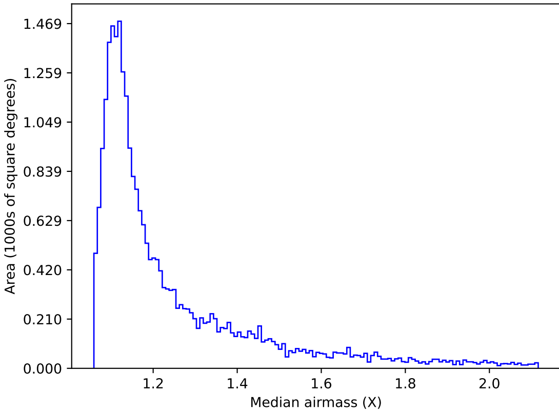
ddf_loaded_fl1_v3.4_10yrs Yr 1 r band: Median airmass
