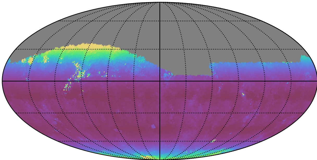
ddf_loaded_fl1_v3.4_10yrs Yr 1 i band: Median airmass
