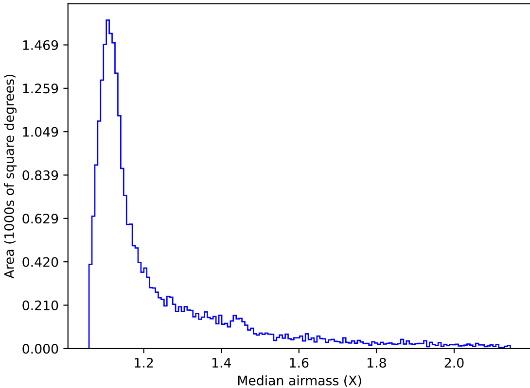
ddf_loaded_fl1_v3.4_10yrs Yr 1 i band: Median airmass
