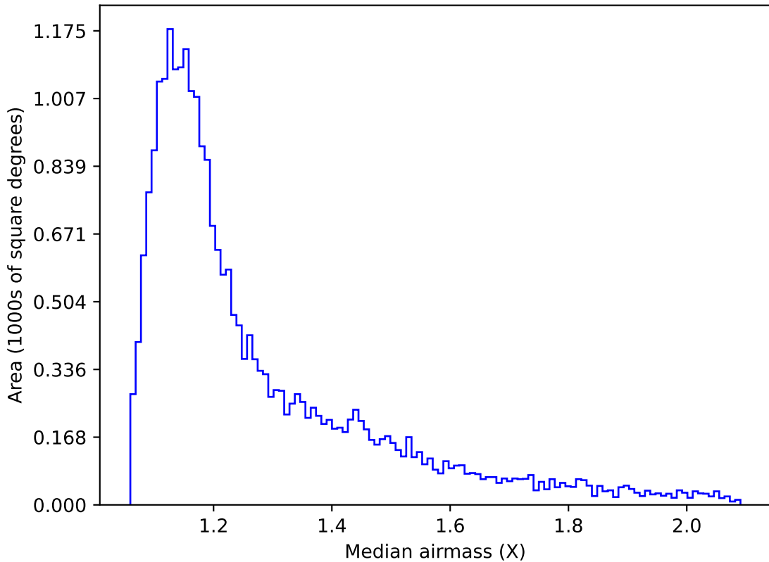
ddf_loaded_fl1_v3.4_10yrs Yr 1 g band: Median airmass
